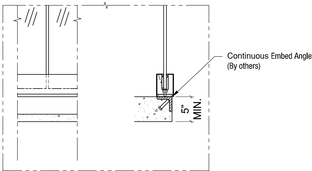
Welded @ Embed Angle - $$$
