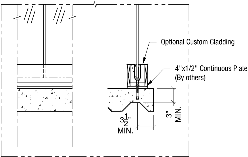
Anchored to Concrete Slab on Deck - $$$
