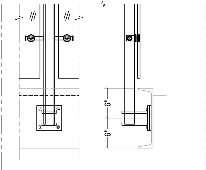
Welded @ Steel Channel - $$ Detail# BLA-F03
