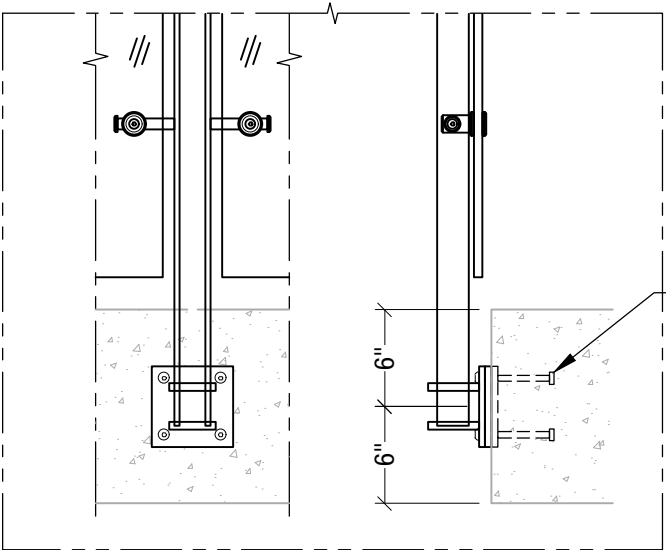
Welded @ Embed Plate - $$ Detail# BLA-F02
