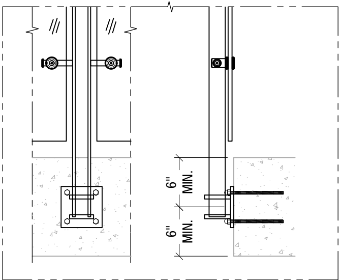
Anchored to Concrete 1 - $$$ Detail# BLA-F01
