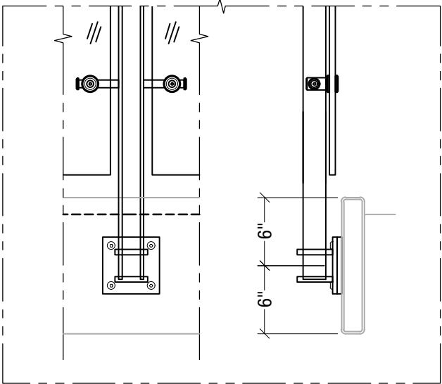
Welded @ Steel Tube - $$ Detail# BLA-F04
